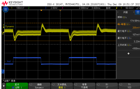
Figure 4, 25% - 50% load dynamic
